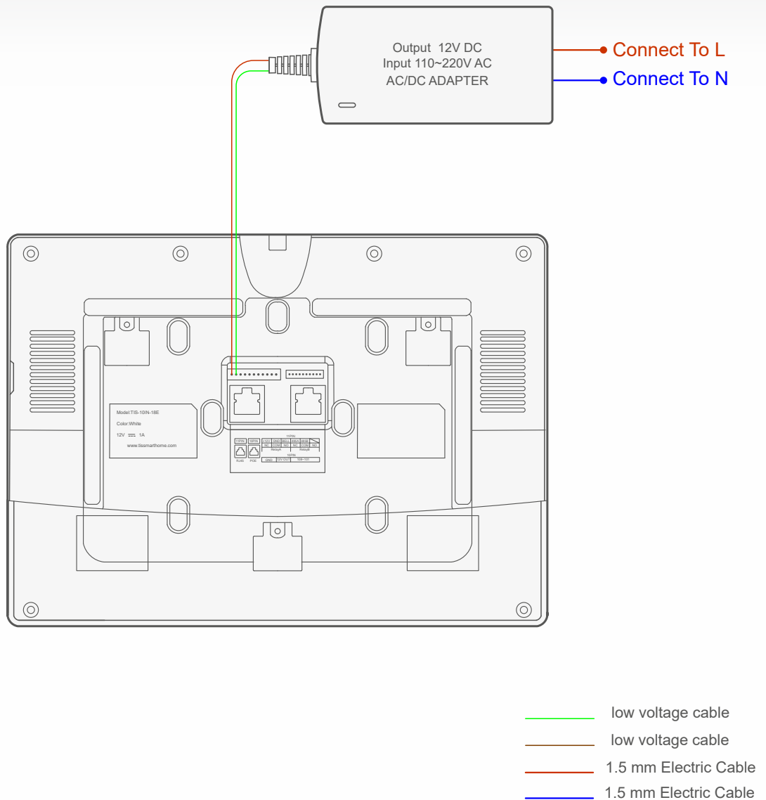
▲ Figure 1: TIS-10IN-18E & Power Supply Connection Diagram
