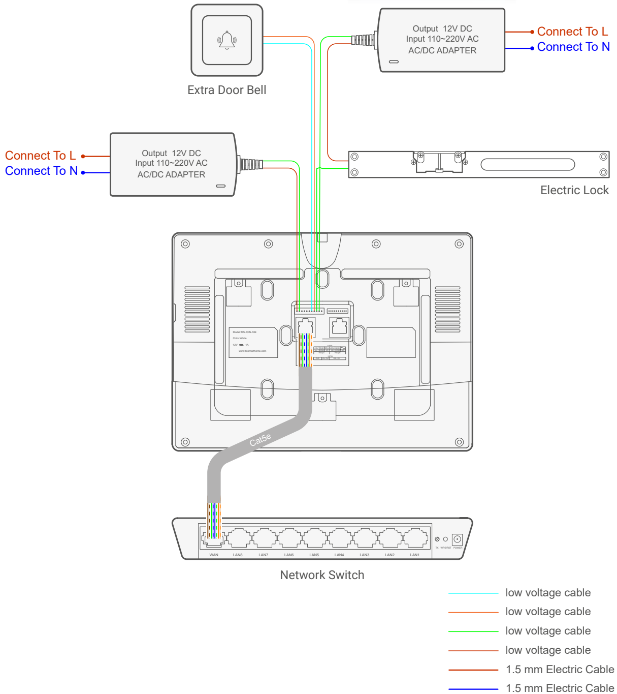
▲ Figure 6: TIS-10IN-18E, Electric Lock & Extra Bell Unit Connection Diagram
