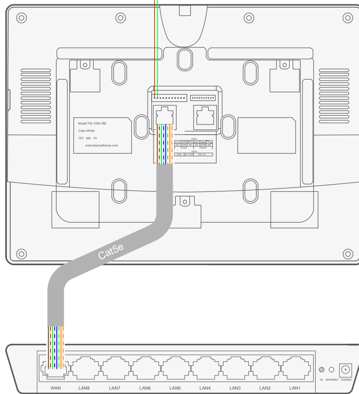
Network Switch
