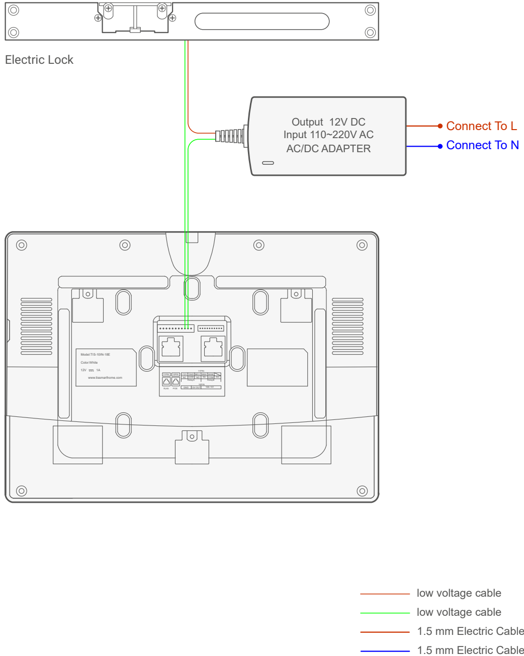
▲ Figure 4: TIS-10IN-18E & Electric Lock Connection Diagram
