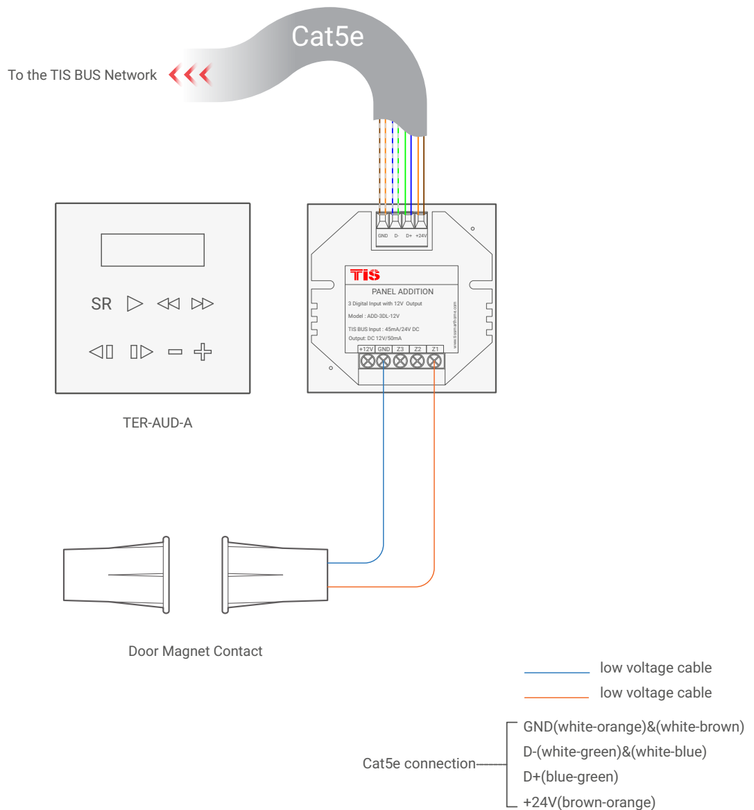
▲ Figure 5: TER-AUD-A & ADD-3DL-12V Magnetic Door Contact Connection Diagram
