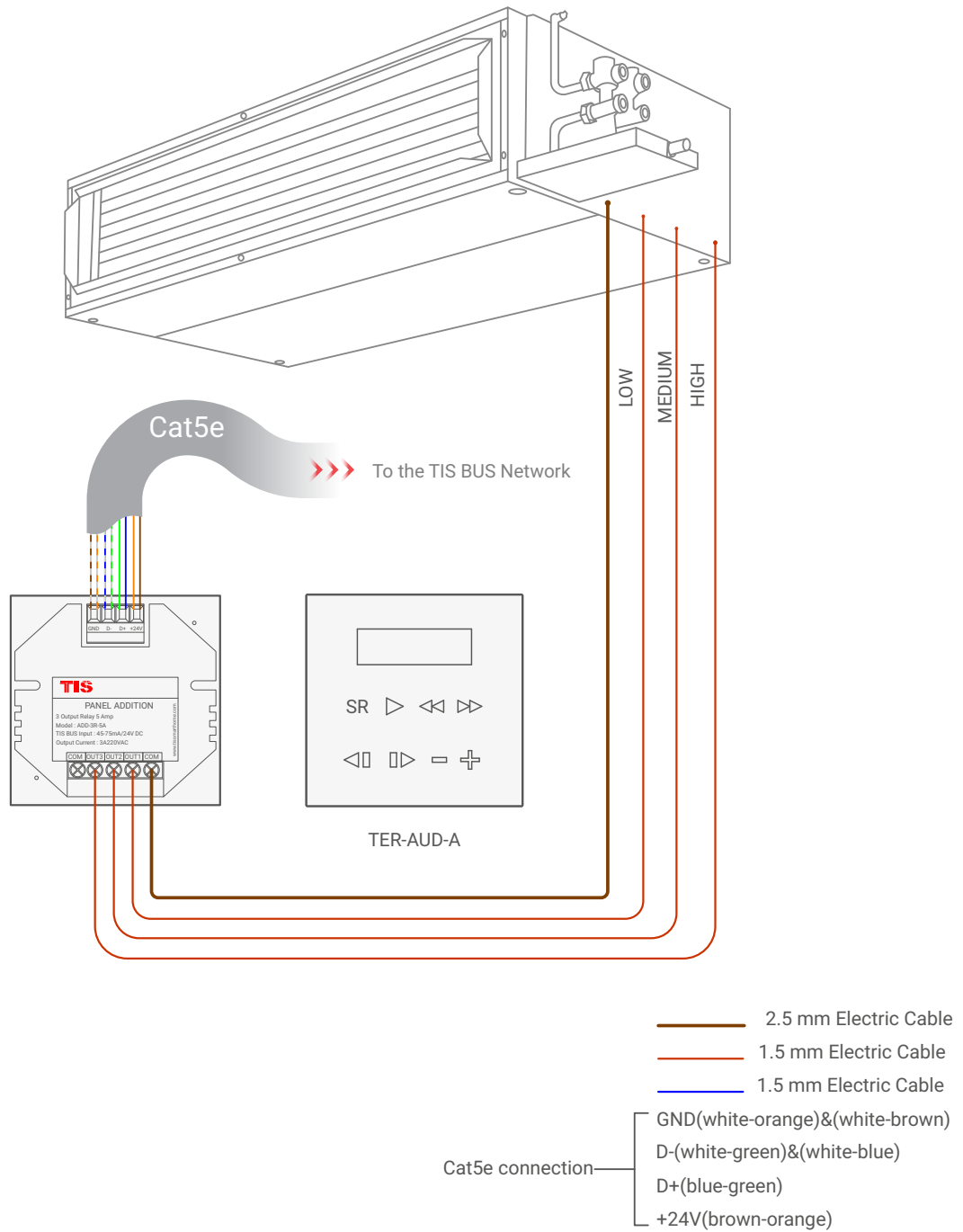
▲ Figure 3: TER-AUD-A & ADD-3R-5A FCU Connection Diagram
