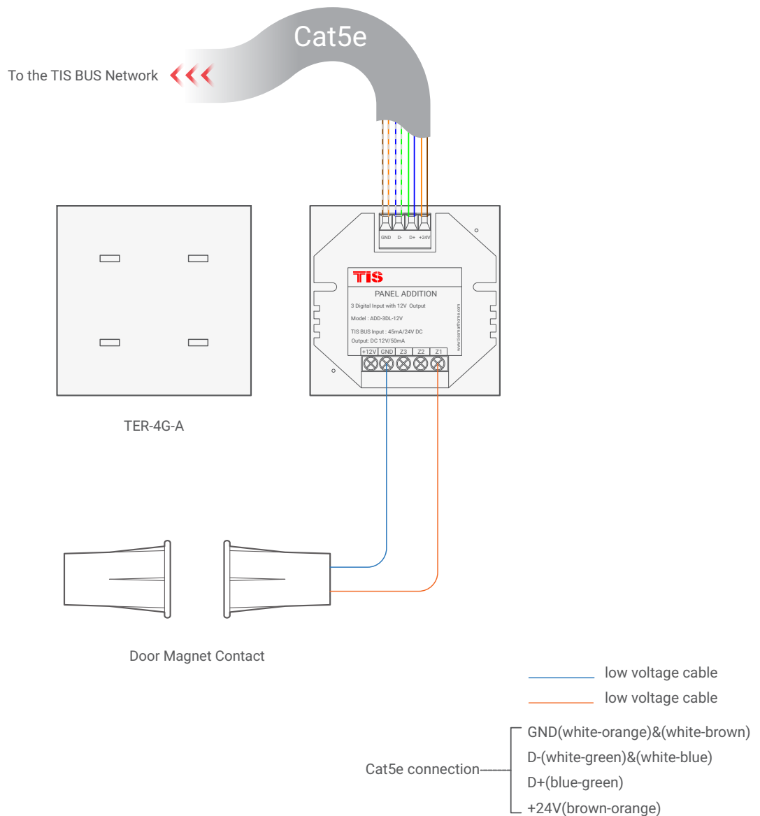
▲ Figure 5: TER-4G-A & ADD-3DL-12V Magnetic Door Contact Connection Diagram
