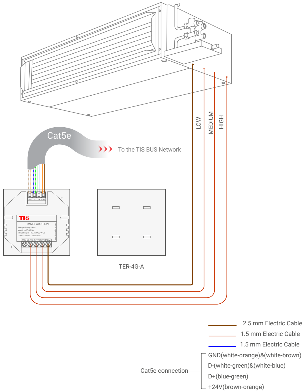
▲ Figure 3: TER-4G-A & ADD-3R-5A FCU Connection Diagram
