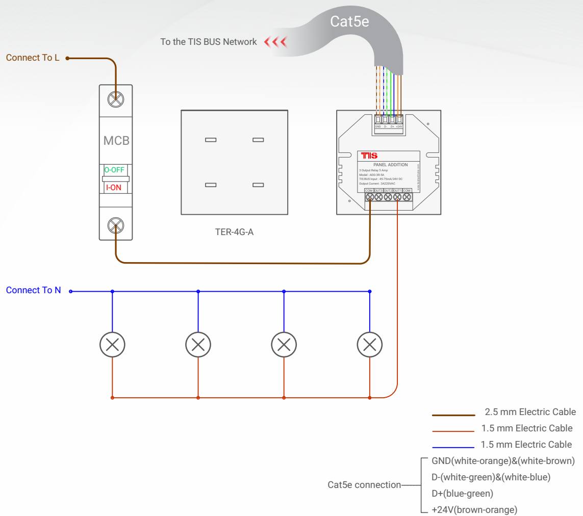
▲ Figure 1: TER-4G-A & ADD-3R-5A Lights Connection Diagram
