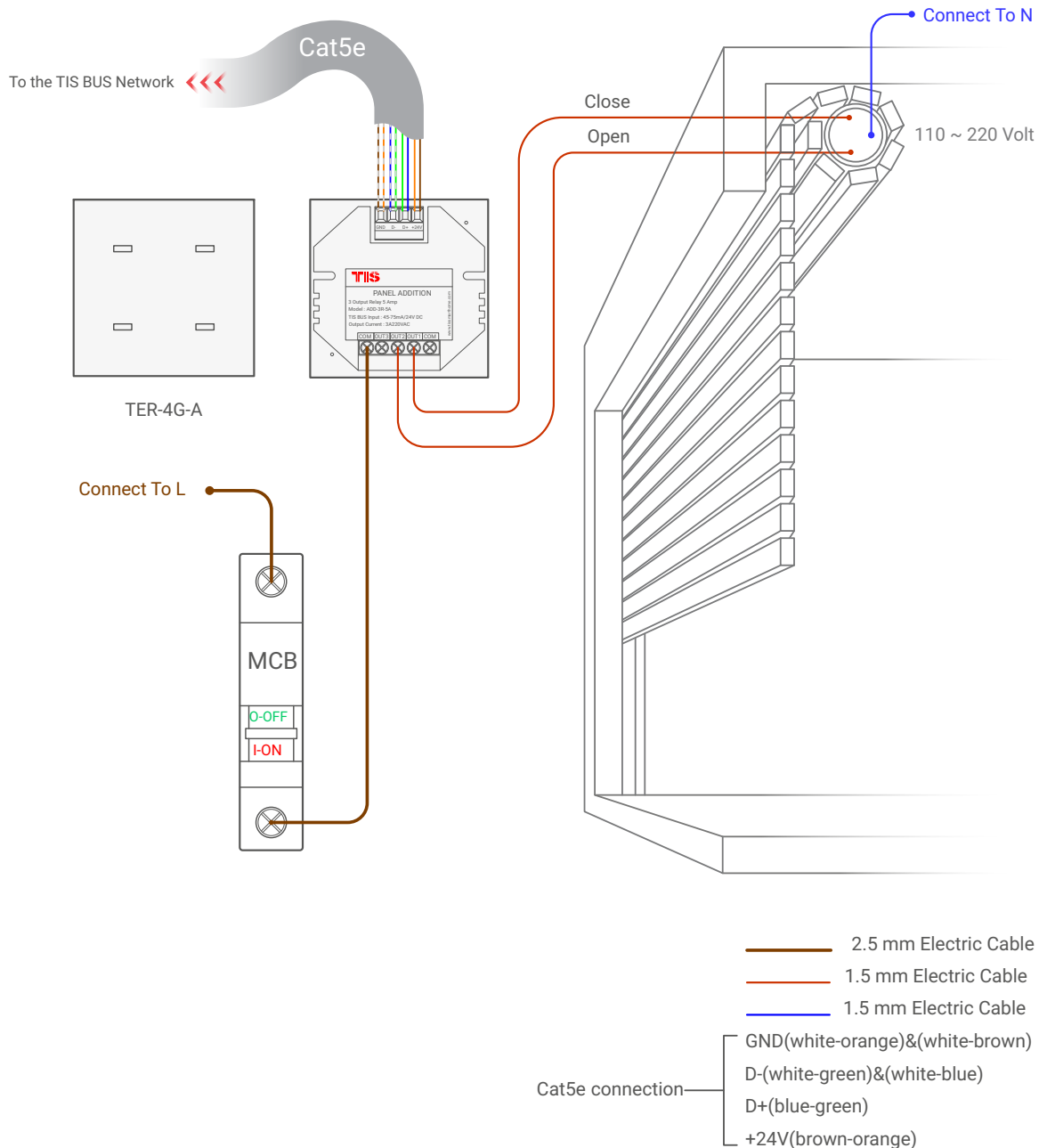
▲ Figure 2: TER-4G-A & ADD-3R-5A Motors Connection Diagram
