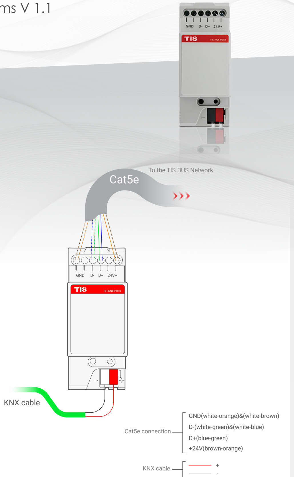
▲ Figure 1: TIS BUS-KNX Converter Configuration Diagram
